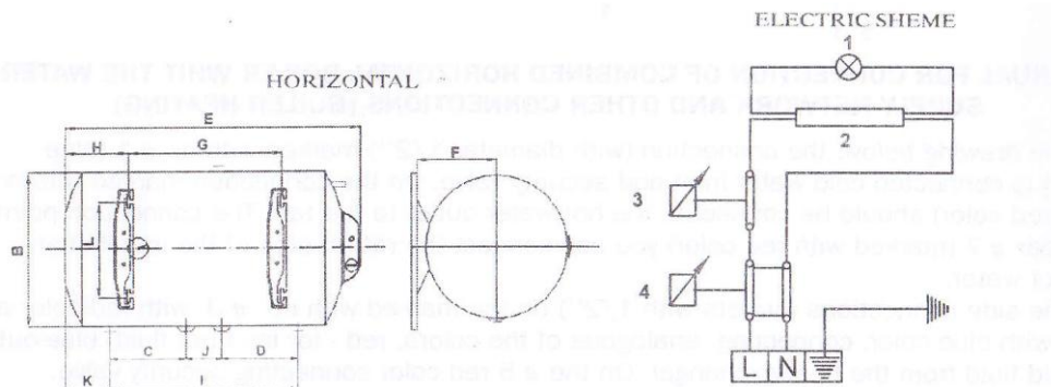
ELECTRIC SCHEME
